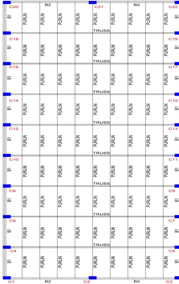
TRUSS BOTTOM PLAN
